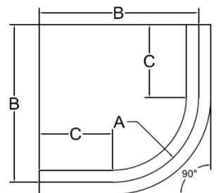
90° dimensional drawing
